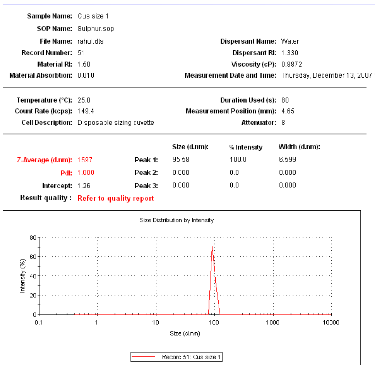
Figure 6.7: The graph of intensity vs. size for 2nd run
