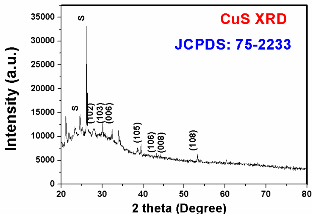
Figure 6.9: The graph of intensity vs. ( 2\theta ) plotted from data obtained from XRD analysis
