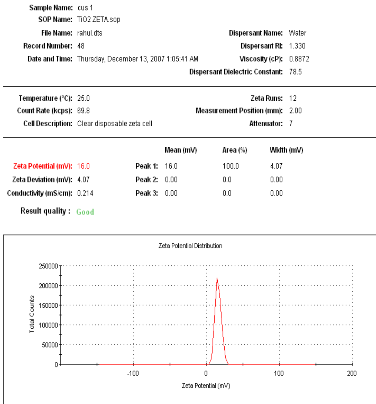
Figure 6.8: The zeta potential distribution graph
