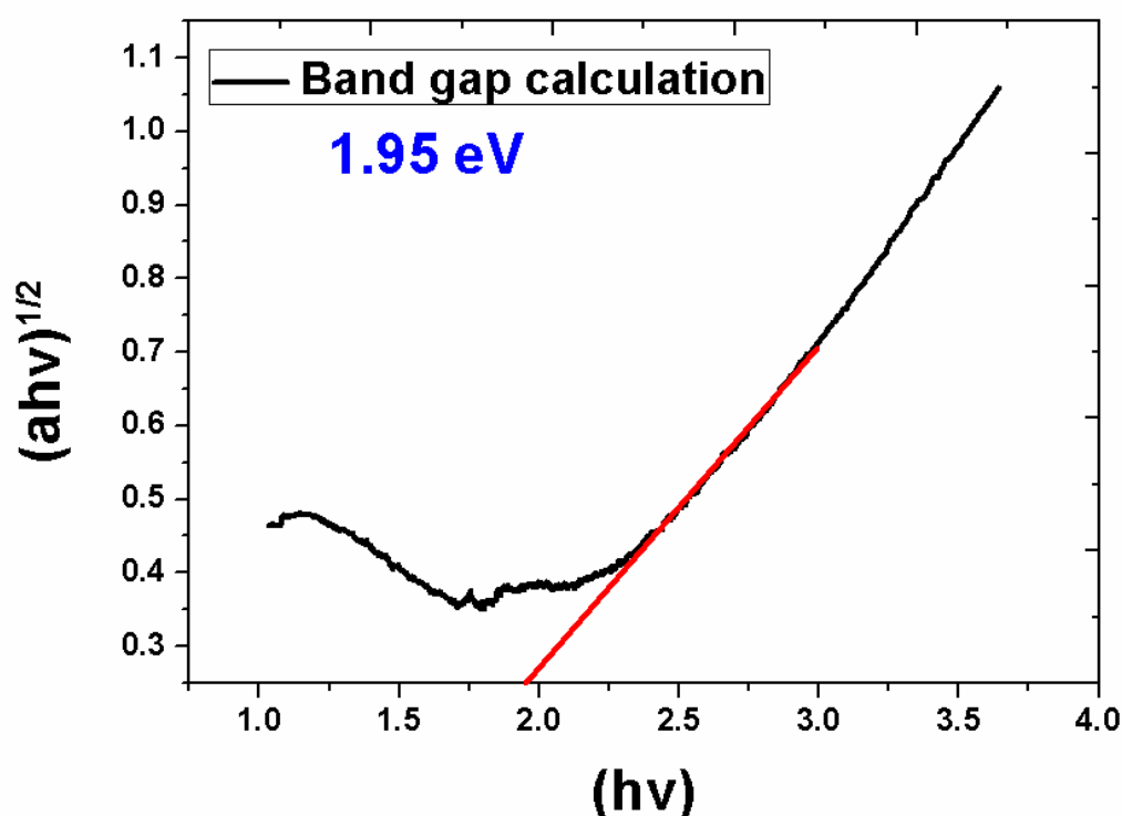
Figure 6.3: The plot for band gap
