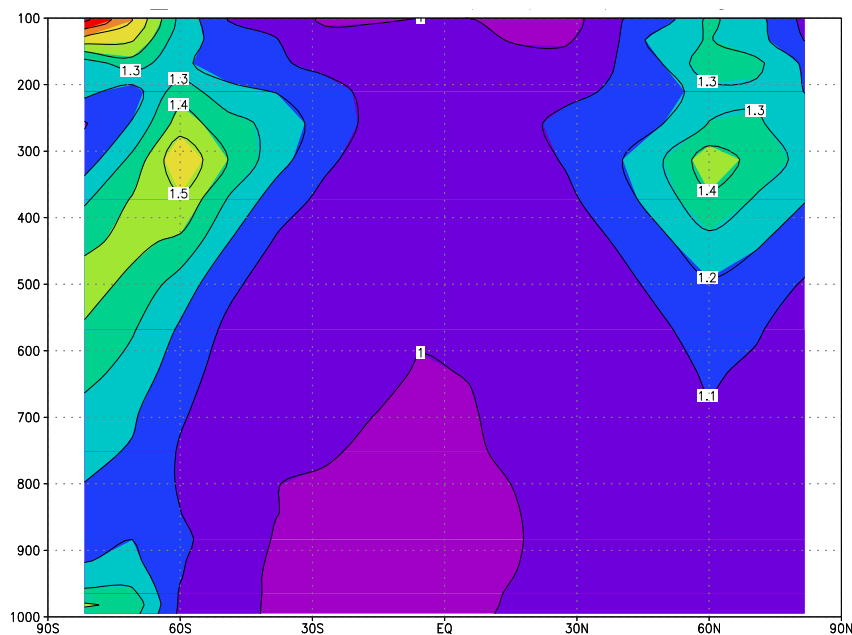
Fig. 12. Ratio of \text{OH}:\text{HO}_2 in scenario “high lat” to \text{OH}:\text{HO}_2 in scenario “no hal”. The numbers are zonally and annually averaged. The ordinate is the \sigma -level multiplied by 1000 which is approximately the pressure in hPa and the abscissa is latitude in degrees. Note that 24h averages are plotted.
