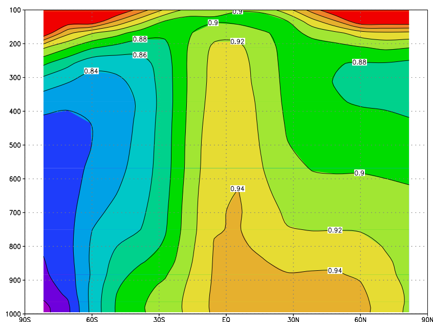
Fig. 9. Ratio of \text{O}_3 in scenario “high lat” to \text{O}_3 in scenario “no hal”. The numbers are zonally and annually averaged. The ordinate is the \sigma -level multiplied by 1000 which is approximately the pressure in hPa and the abscissa is latitude in degrees. Note that 24h averages are plotted.
