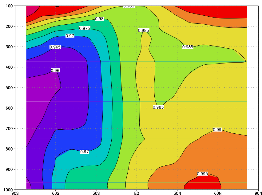
Fig. 11. Ratio of \text{O}_3 in scenario “strat” to \text{O}_3 in scenario “no hal”. The numbers are zonally and annually averaged. The ordinate is the \sigma -level multiplied by 1000 which is approximately the pressure in hPa and the abscissa is latitude in degrees. Note that 24 h averages are plotted.
