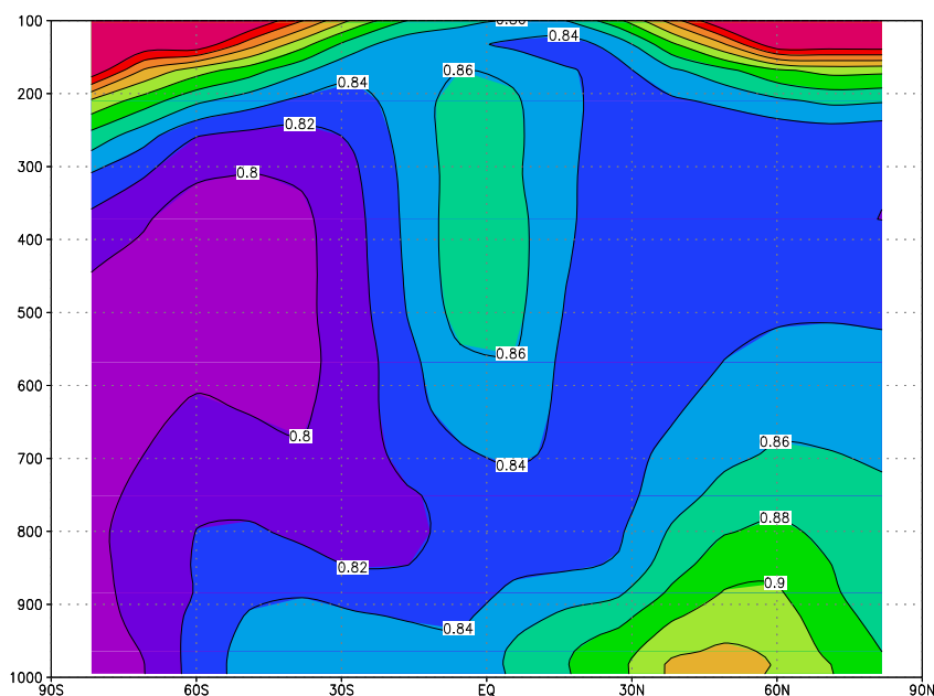
Fig. 10. Ratio of \text{O}_3 in scenario “tropics” to \text{O}_3 in scenario “no hal”. The numbers are zonally and annually averaged. The ordinate is the \sigma -level multiplied by 1000 which is approximately the pressure in hPa and the abscissa is latitude in degrees. Note that 24h averages are plotted.
