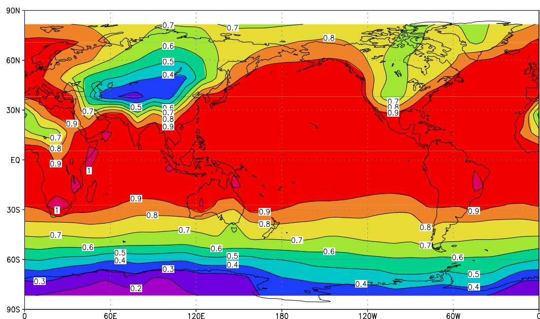
Fig. 15. Ratio of the vertical column of DMS for the scenario “high lat” to scenario “no hal” (annually averaged). The ordinate is latitude in degrees and the abscissa is longitude in degrees. Seasalt aerosol is not explicitly included as a source for BrO therefore the reductions in DMS are lower limits.
