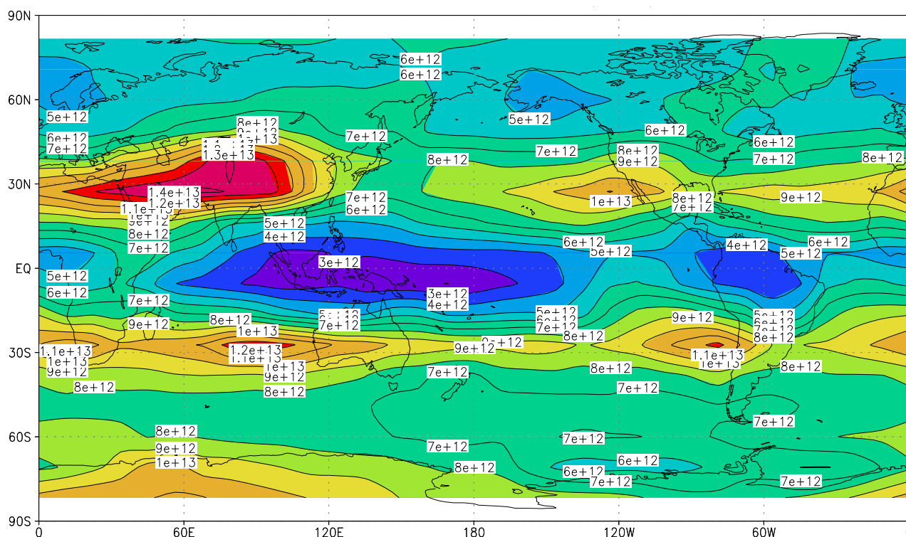
Fig. 7. Annually averaged tropospheric vertical column of BrO (in molec cm -2 ) for the scenario “high lat”. We used the WMO definition for the determination of the tropopause. Note that 24h averages are plotted. The ordinate is latitude in degrees and the abscissa is longitude in degrees.
