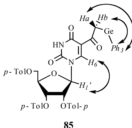
Figure 18. Important NOE interactions observed for 5-[2-(triphenylgermyl)acetyl]-2',3',5'-tri- O - p -toluyuridine.
