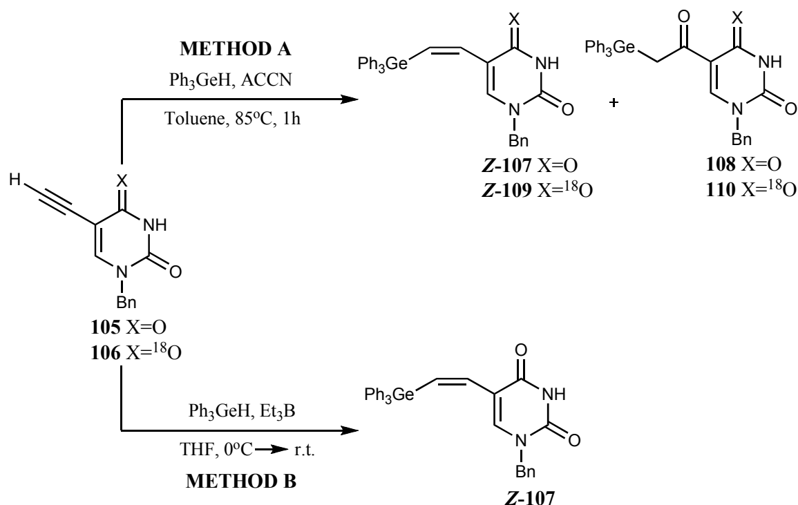
Scheme 30. Hydrogermylation of 1- N -benzyl-5-ethynyluracil and its 4-[ 18 O]-labeled analogue.
