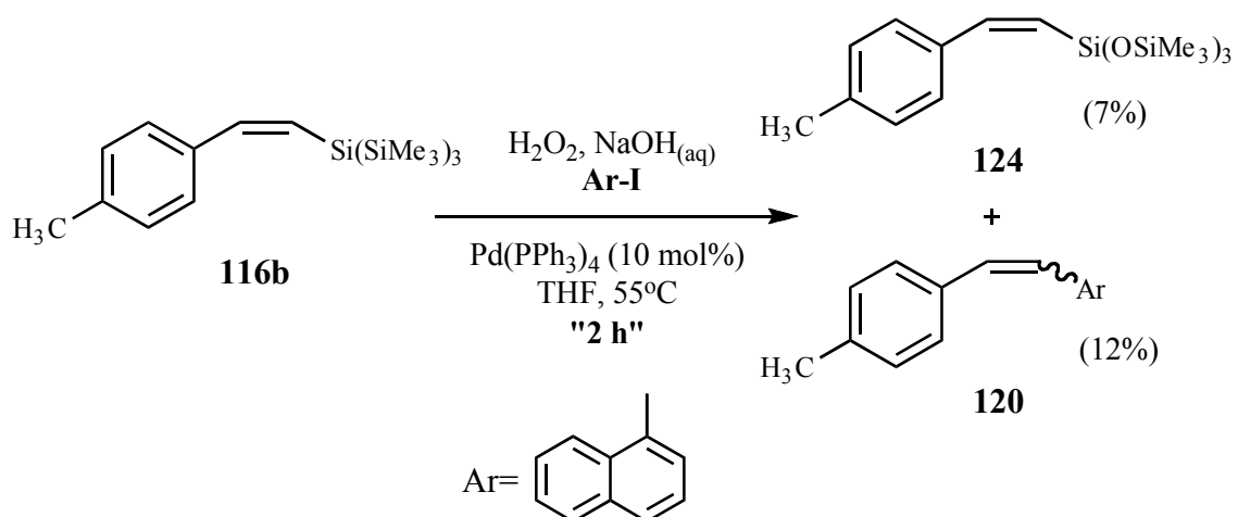
Scheme 38. The Formation of (Z)-2-(4-methylphenyl)-1-[tris(trimethylsiloxy)silyl]ethene during the coupling with (Z)-tris(trimethylsilyl)silanes.
