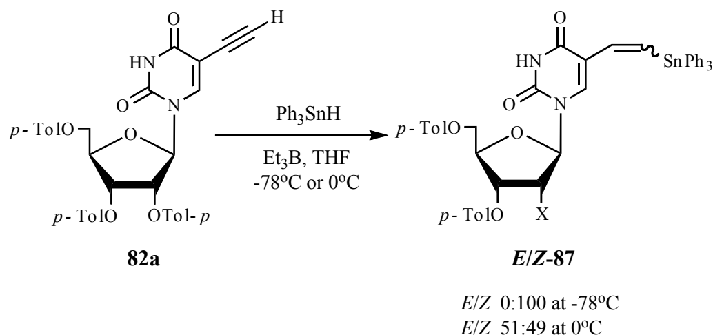
Scheme 26. \text{Et}_3\text{B} -promoted radical hydrostannylation of p -toluylyl-protected 5-ethynyluridine analogues.
