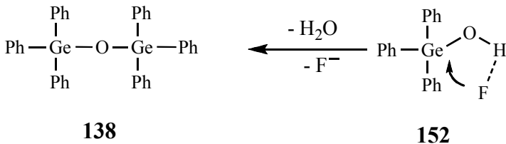
Scheme 52. Proposed pathway for the activation of chloro(triphenyl)germane with TBAF.
