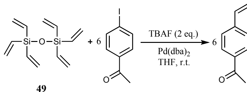
Scheme 14. Coupling of hexavinylidisiloxane with 4-iodoacetophenone. 130
