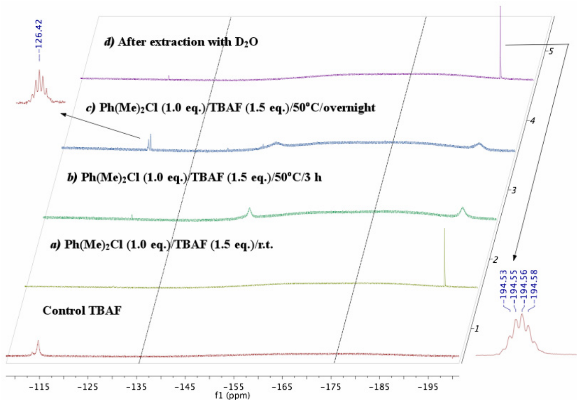
Figure 22. ^{19}\text{F} NMR analyses of the reaction of chloro(dimethyl)phenylgermane with TBAF in benzene- d_6 .
