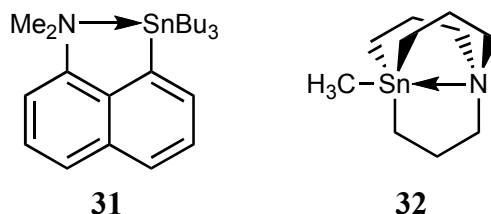
Figure 11. Hypervalent organostannates by internal coordination employed in Pd-catalyzed cross-coupling reactions.
