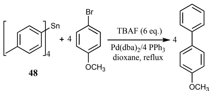
Scheme 13. Coupling of tetra( p -tolyl)tin with 4-bromoanisole. 80
