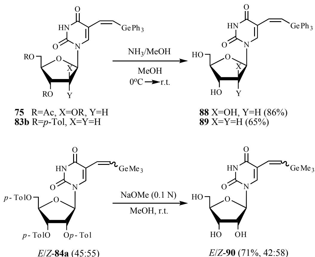
Scheme 27. Deprotection of acetyl and p -toluyyl-protected 5-[2-(germyl)ethenyl]uridine analogues.
