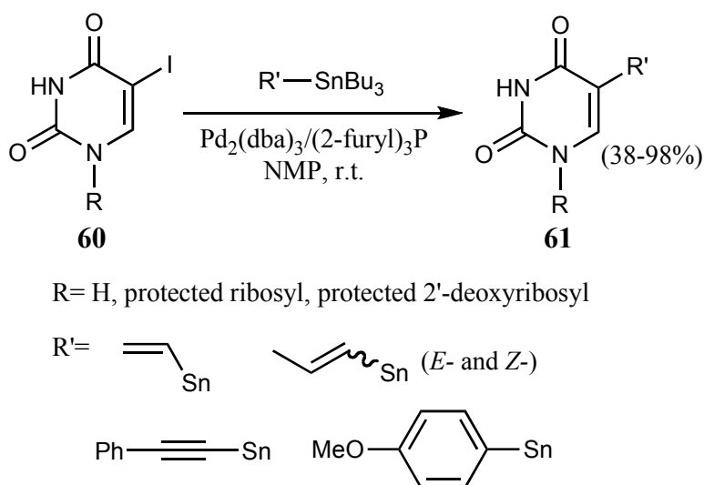
Scheme 19. Coupling of 5-iodouracil, uridine, and 2'-deoxyuridine analogues with different unsaturated organotin compounds. 152
