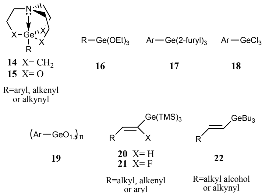
Figure 10. Organogermanes employed in Pd-catalyzed cross-coupling reactions.
