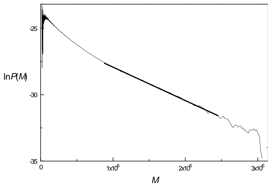
Figure 5.9: \ln P(M) plot for VAc emulsion polymerization, 62°C, 23% conversion, [persulfate] = 7.0 \times 10^{-4} M. The region of the plot used in equation 5.3 is shown in bold.
