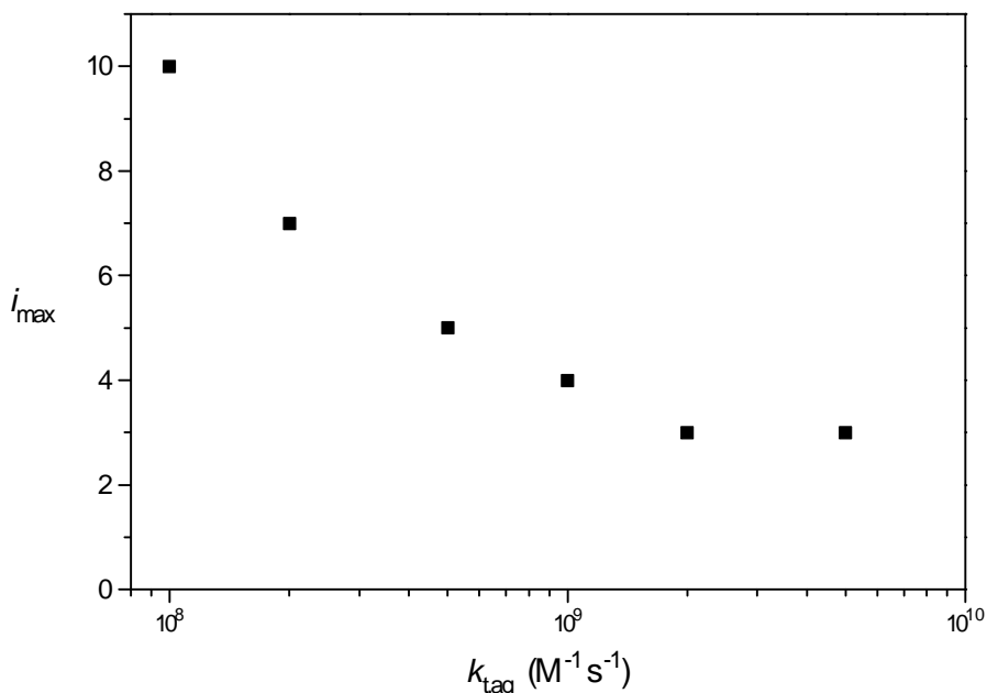
Figure 4.15: Degree of polymerization, i_{max} , below which more than 95% of aqueous-phase oligomeric radicals terminate (i.e. value of i where P_{term}^i > 0.05 , equation 4.20) as function of k_{taq} . Simulation based on equations 4.9 – 4.17, termination calculated from equation 4.18. [S_2O_8^{2-}] = 0.1 \text{ M} , 50^\circ\text{C} , [VAc] = 0.05 \text{ M} .
