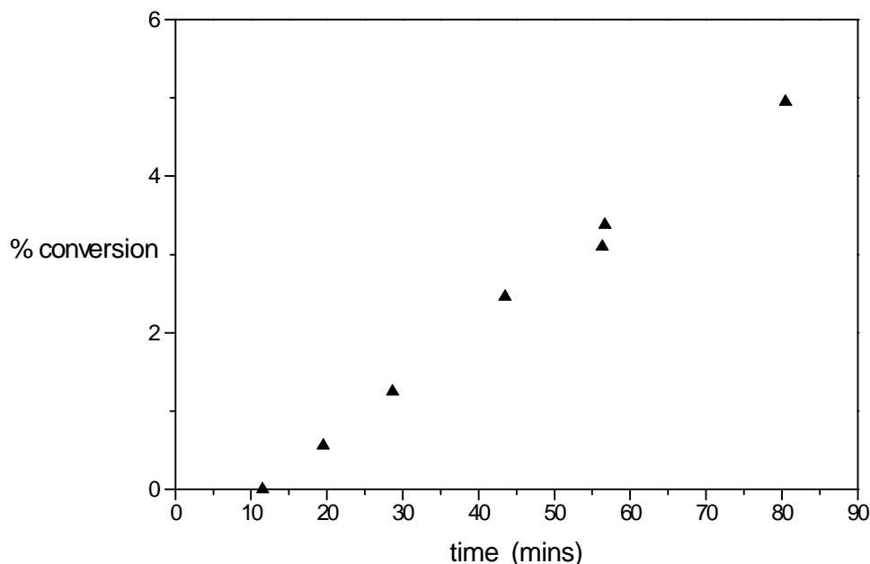
Figure 5.1: Typical plot of conversion as function of time for bulk polymerization of VAc, 64°C, [AIBN] = 6.4 \times 10^{-5} \text{ M} .
