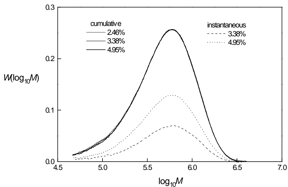
Figure 5.3: MWDs for bulk VAc polymerization, 64°C, [AIBN] = 6.4 \times 10^{-5} \text{ M} .
