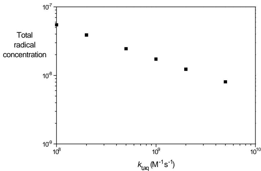
Figure 4.14: Calculated total radical concentration for solution polymerization of VAc (expt. A1) as function of k_{t,aq} . Simulation based on equations 4.9 – 4.17. [S_2O_8^{2-}] = 0.1 M, 50^\circ C , [VAc] = 0.05 M.
