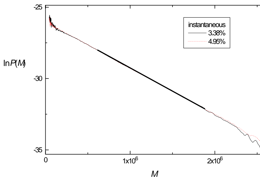
Figure 5.4: \ln P(M) plot for bulk VAc polymerization, 64°C, [AIBN] = 6.4 \times 10^{-5} \text{ M} . The region of the plot used in equation 5.3 is shown in bold.
