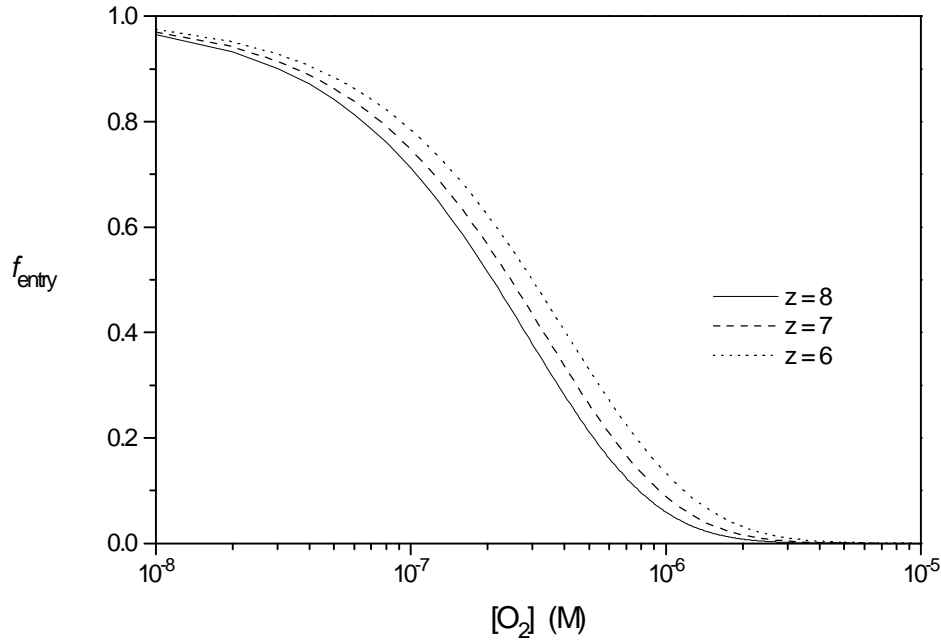
Figure 4.7: f_{\text{entry}} calculated as function of [\text{O}_2] and z (equation 4.6) for VAc emulsion polymerization in interval II at 50°C, k_p = 6.7 \times 10^{-3} \text{ M}^{-1} \text{ s}^{-1} , [\text{M}_{\text{aq}}] = 0.3 \text{ M} , k_{t,\text{O}_2} = 10^9 \text{ M}^{-1} \text{ s}^{-1} .
