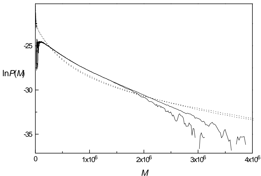
Figure 5.2: Instantaneous \ln P(M) plots, (·····) Waters 10^6 , 10^5 , 10^4 , and 10^3 Å monodisperse pore size columns, (—) Waters Styragel mixed bed columns. VAc bulk polymerization, 64^\circ\text{C} , [\text{AIBN}] = 6.4 \times 10^{-5} \text{ M} .
