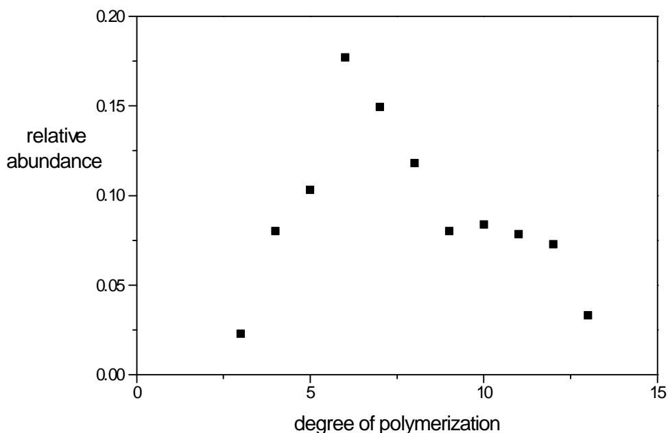
Figure 4.22: Distribution of degree of polymerization of partially hydrolysed oligomers produced under similar conditions to those of Morris and Parts, [S_2O_8^{2-}] = 0.12 M, 50^\circ\text{C} , [\text{VAc}] = 0.05 M, experiment A3.
