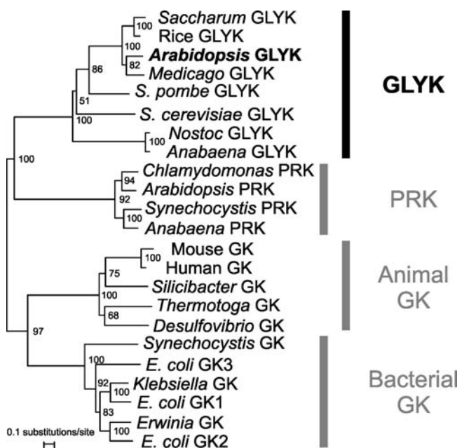
Figure 7. GLYK Represents a Novel Kinase Family Phylogenetically Distinct from Other GK Proteins.
