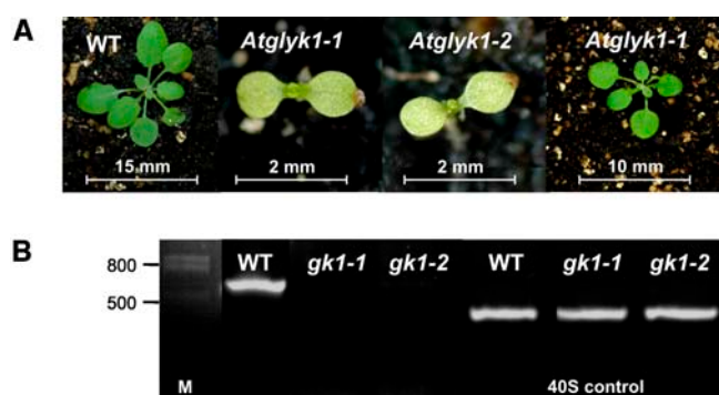
Figure 5. GLYK Is Indispensable for Normal Plant Development and Growth, but This Absolute Requirement Is Relaxed under Elevated \text{CO}_2 .
